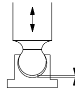
Play at caulking between piston and shoe :
