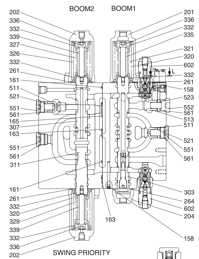
SECTION E-E
