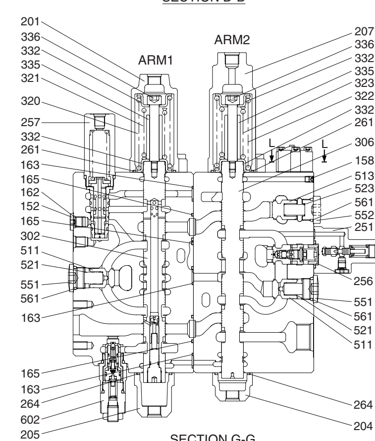
SECTION G-G
