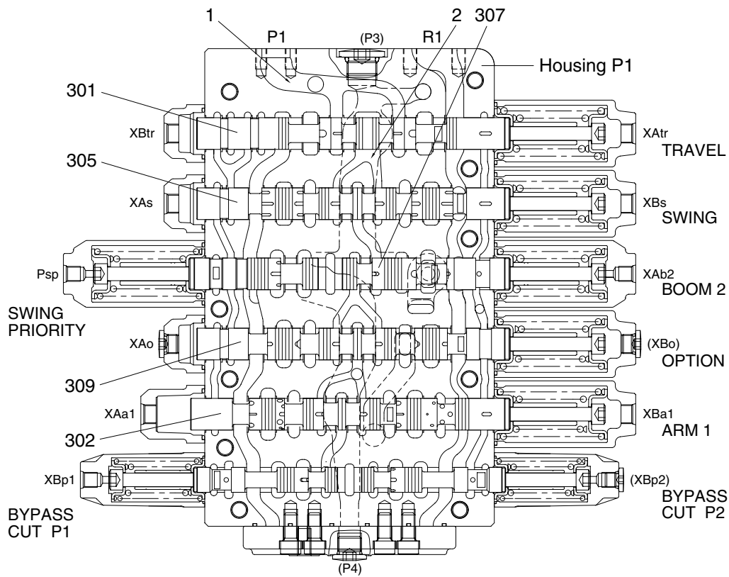
SPOOL SECTION(P1)
