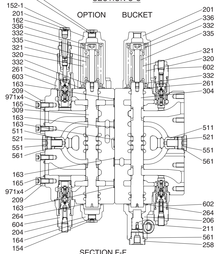
SECTION F-F
