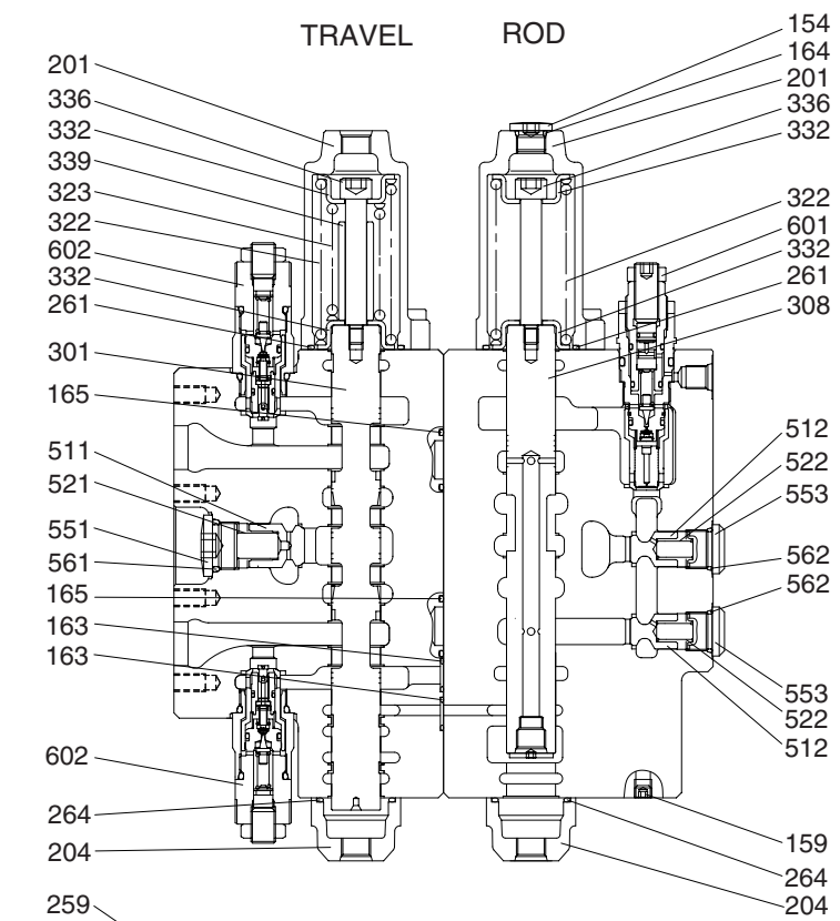
SECTION C-C
