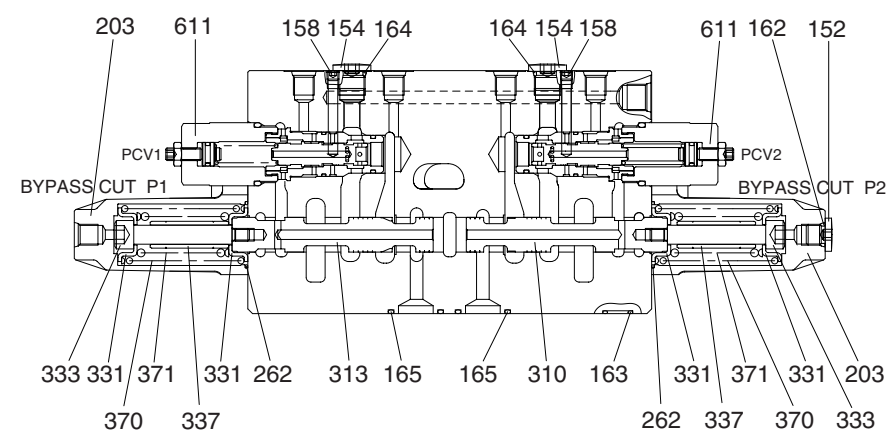
SECTION H-H
