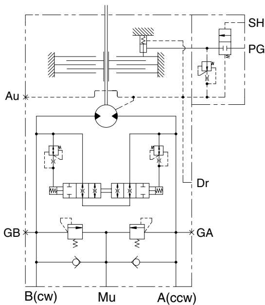
Hydraulic circuit
