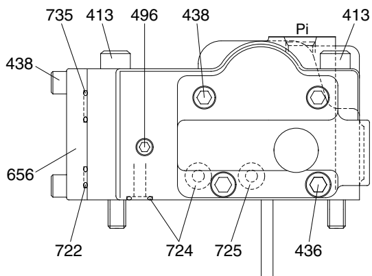
VIEW C
