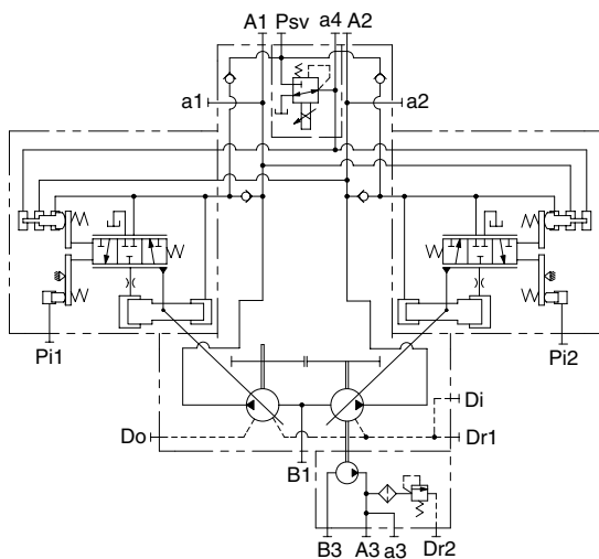
Hydraulic circuit
