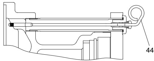
DETAIL K
