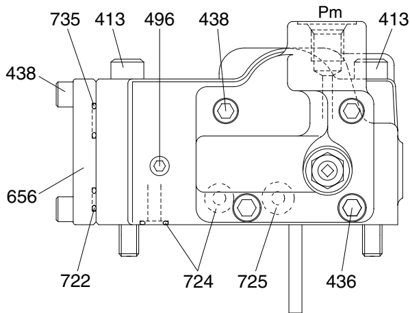
VIEW C
