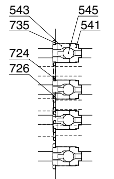
SECTION X-X
