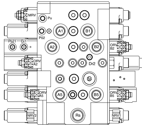
VIEW A
