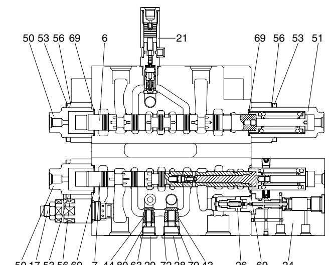
C-C (SWING & BOOM 1)
