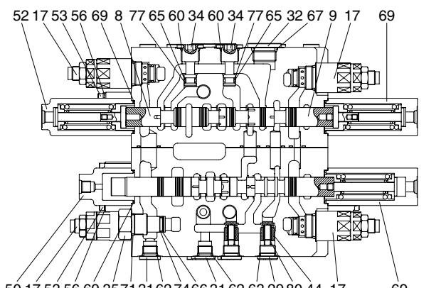
D-D (SWING PRIORITY & BOOM 2 & ARM 2)
