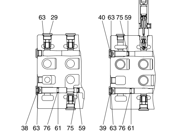
SECTION I-I SECTION H-H
