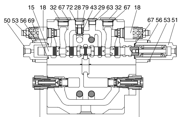
G-G (DOZER & NEGATIVE CONTROL)
