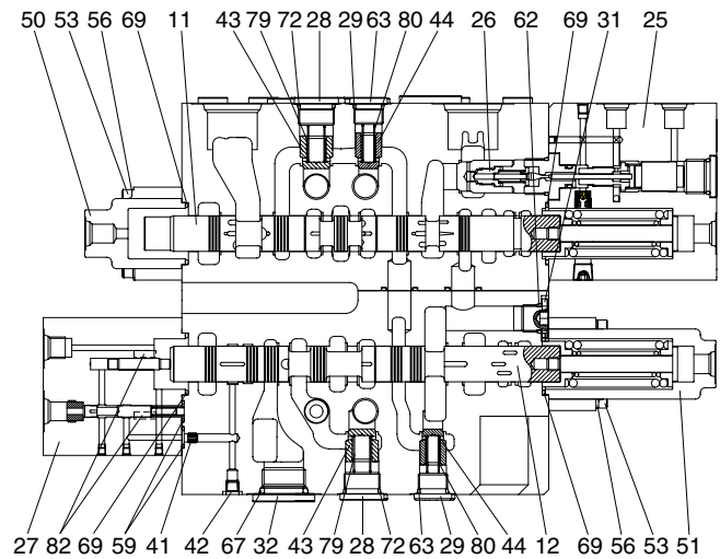
E-E (ARM 1 & ARM REGENERATION / BREAKER)
