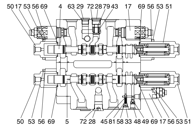
B-B (TRAVEL & OPTION-C)
