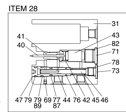
LOCK VALVE - A KIT (BOOM & ARM)
