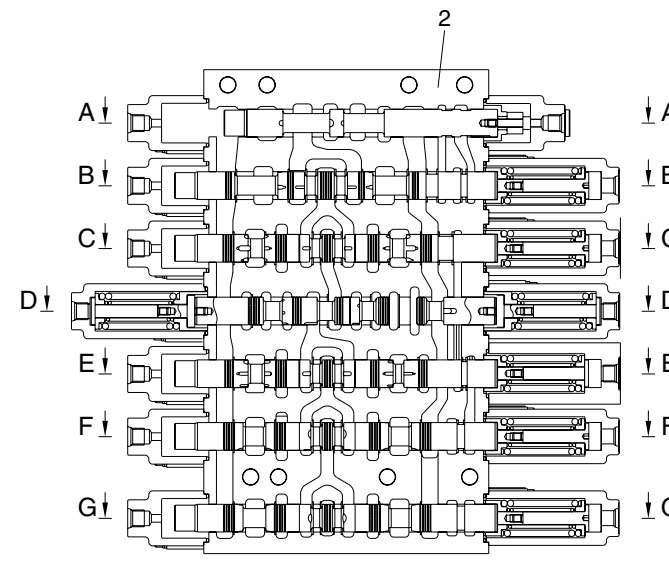
HOUSING P2 SIDE
