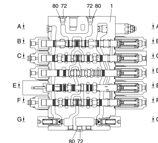
HOUSING P1 SIDE
