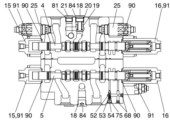
B - B (TRAVEL & DOZER)
