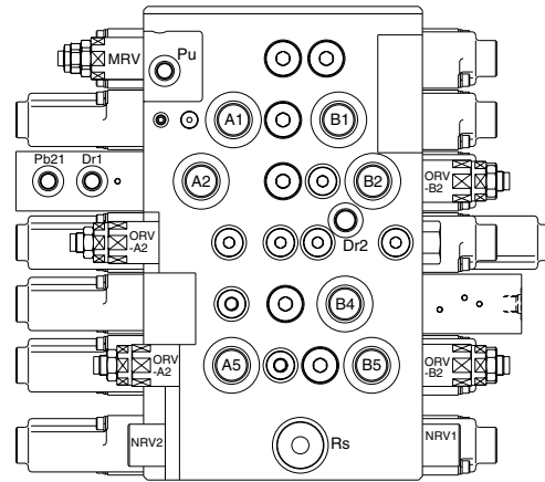
VIEW A
