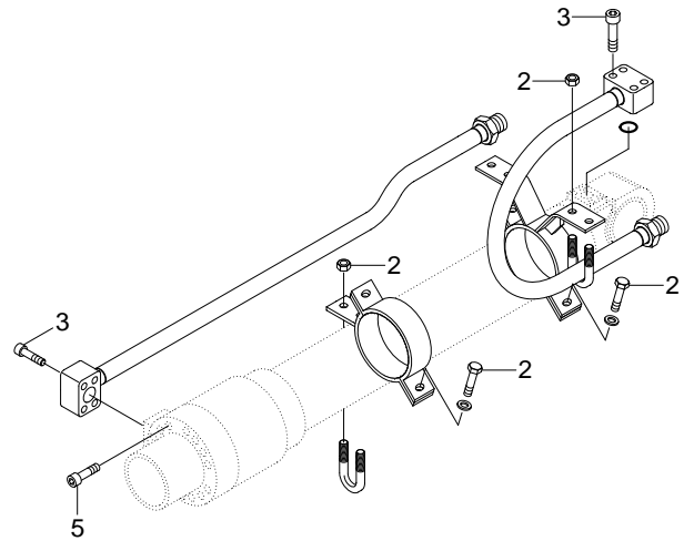
ARM CYLINDER
