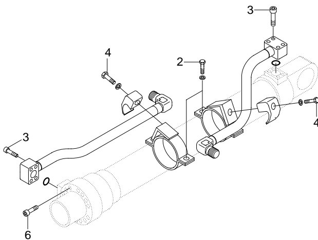
BUCKET CYLINDER
