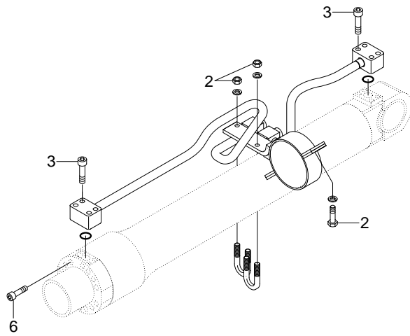
BOOM CYLINDER
