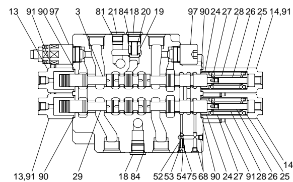
B - B (TRAVEL & DOZER)
