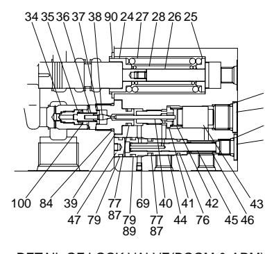
DETAIL OF LOCK VALVE (BOOM & ARM)
