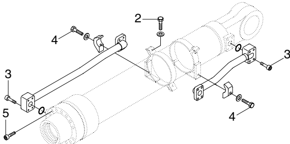
BUCKET CYLINDER
