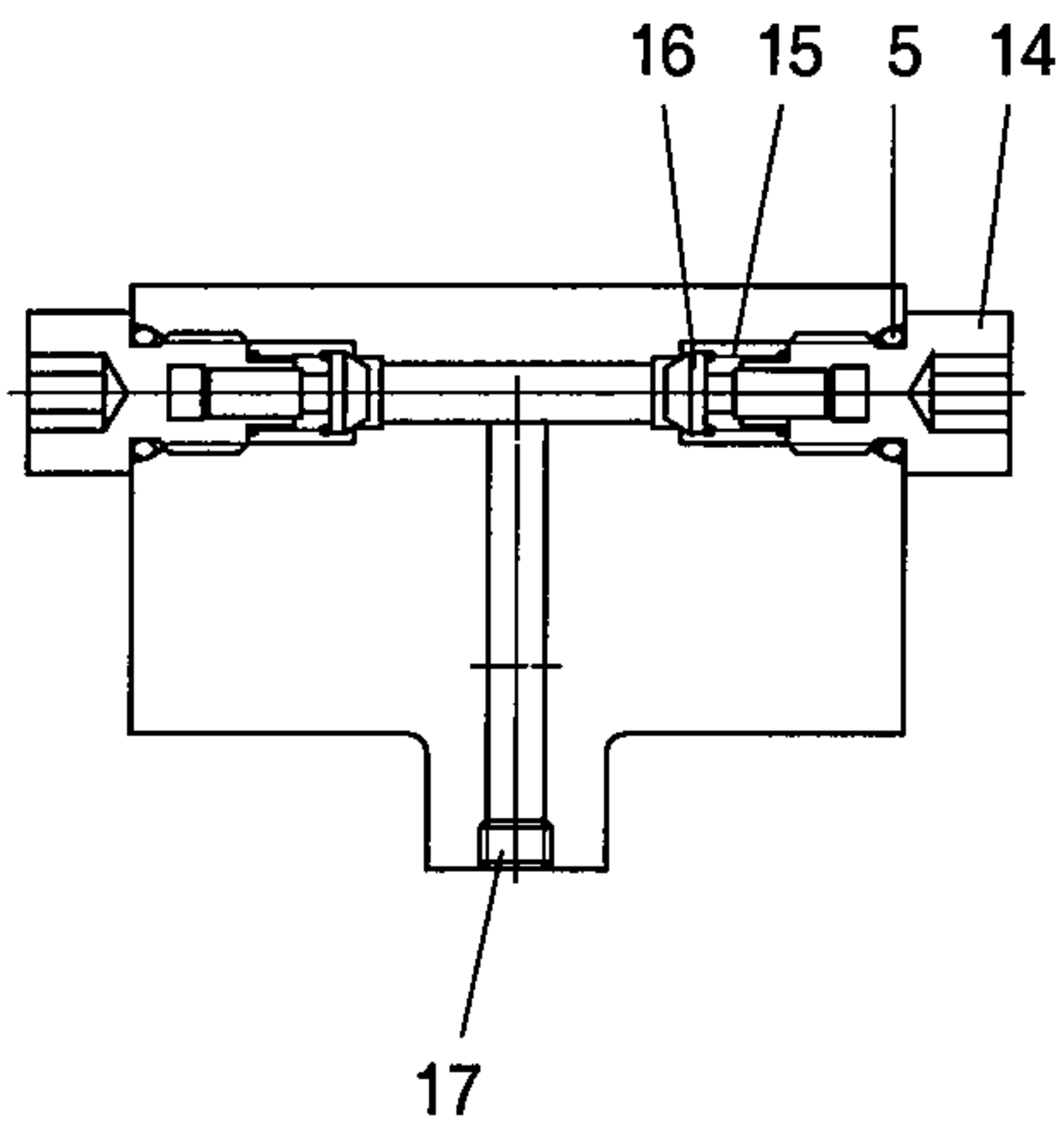
SECTION B-B
