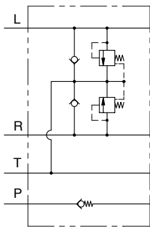
HYDRAULIC CIRCUIT
